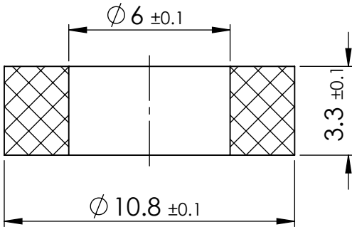
SECTION X-X
